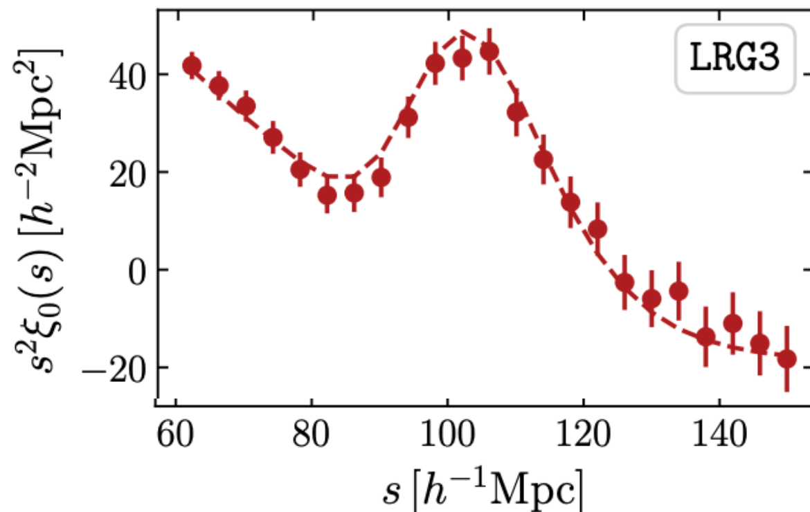
DESI galaxy correlation function
