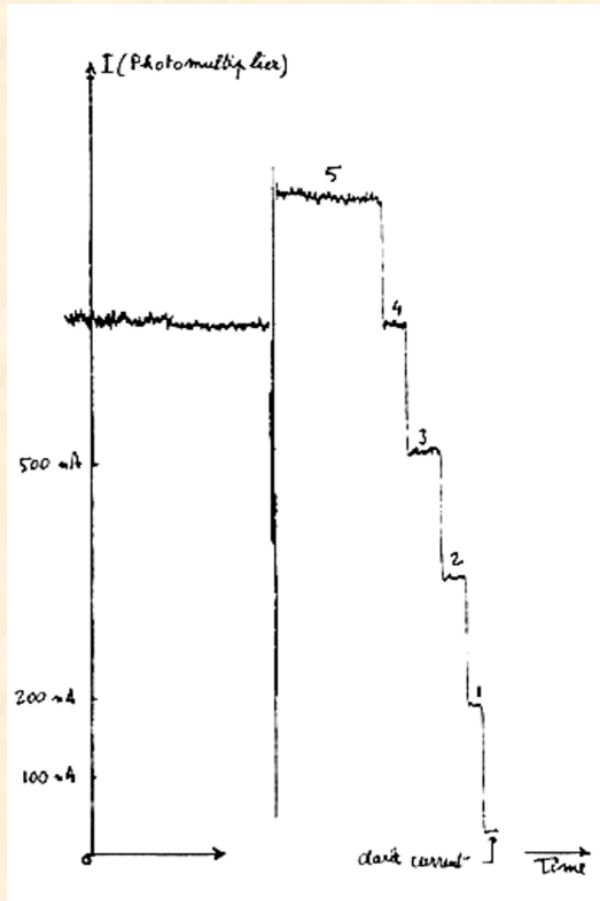
Single electrons
