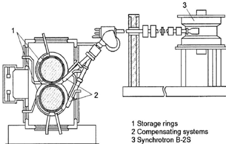
Fig. 2: Layout and photo of the VEP-1 col
