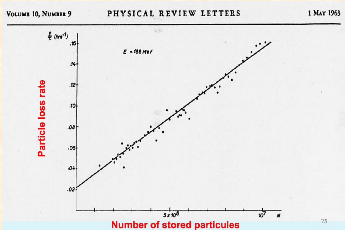
Touschek effect
