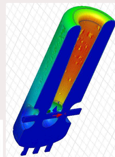
Quarter Wave Resonator, 88 MHz
