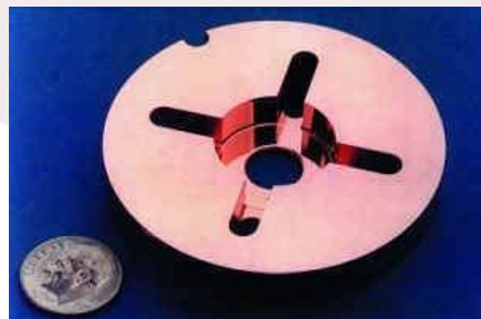
NLC, 11.4 GHz
