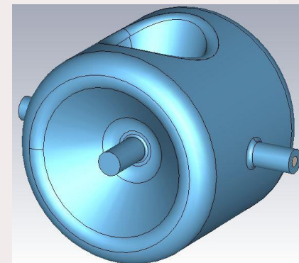
Spoke cavity, 352 MHz
