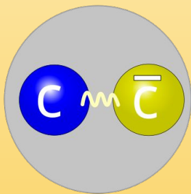
Charmonium
