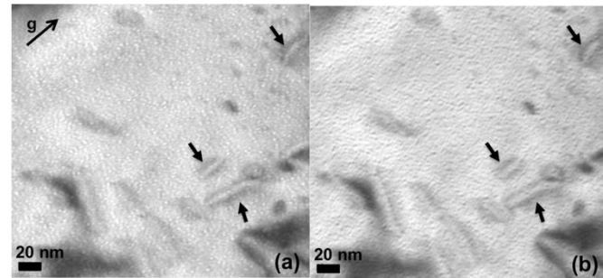
Images recorded in situ at 773 K at 5 dpa; mean bubble size is (2.0 \pm 0.5) nm
