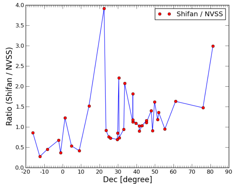
Comparison of sources from Shifan's map and NVSS
