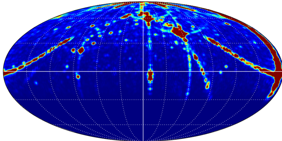
Shifan, center @ (RA=0, Dec=0), smoothed with 1.5°
