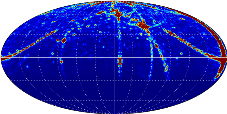
Shifan, center @ (RA=0, Dec=0), smoothed with 1°
