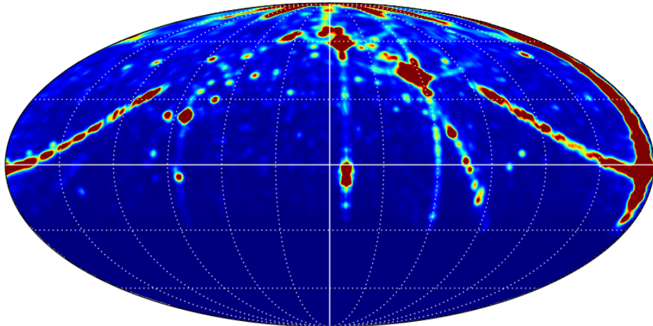
Shifan, center @ (RA=0, Dec=0), smoothed with 2°
